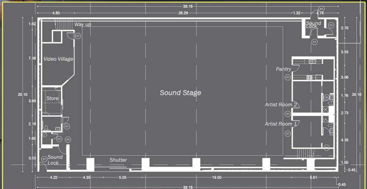
Typical Sound stage Layout
