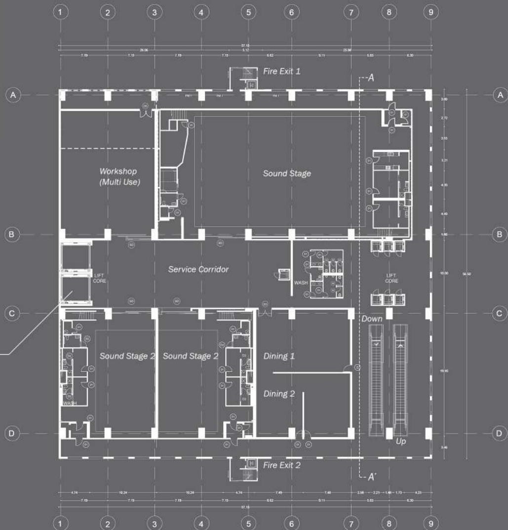
Tower A: Typical Plan
